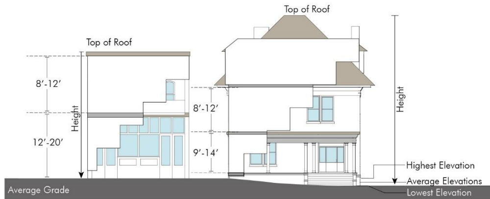
Figure 401-1 Building Height and Building Stories
